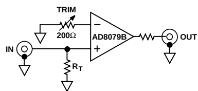
Optional Gain Trim ( G = +2 \rightarrow +2.2 )
